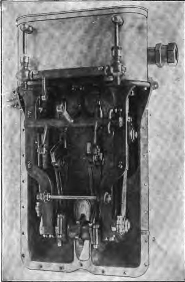
FIG. 251.—Steam Engine of the "Victor" Carriage, showing front of casing removed, also one tube-trunnion for hanging to the body frame.
